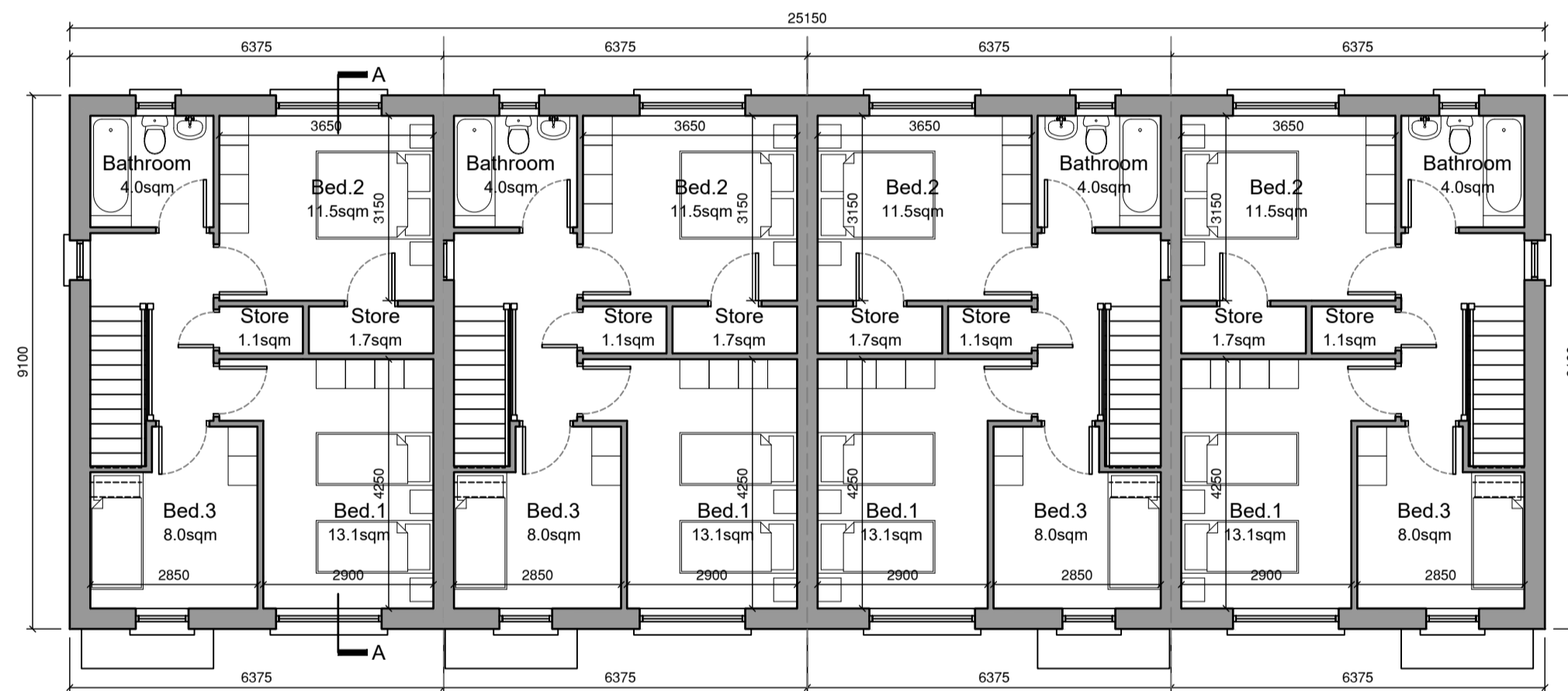
First Floor Plan Area 49.1sqm
