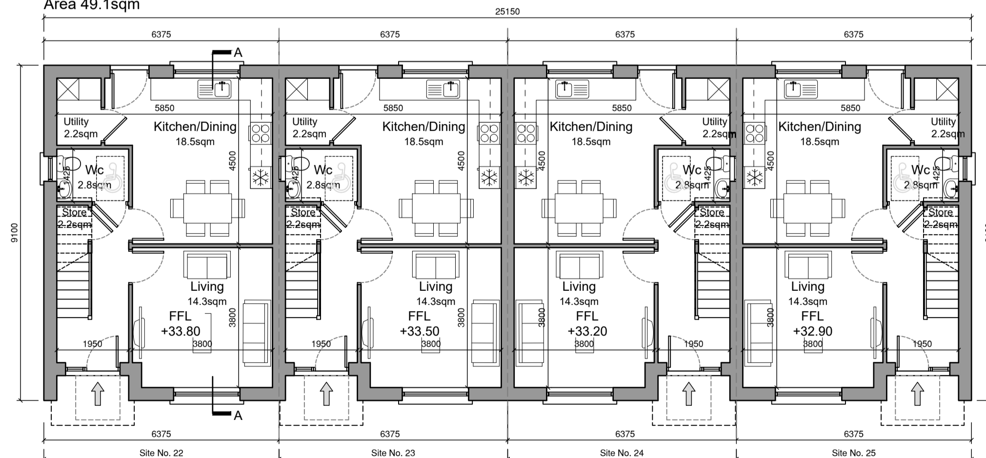
Ground Floor Plan Area:47.6sqm Total Floor Area 96.7sqm
